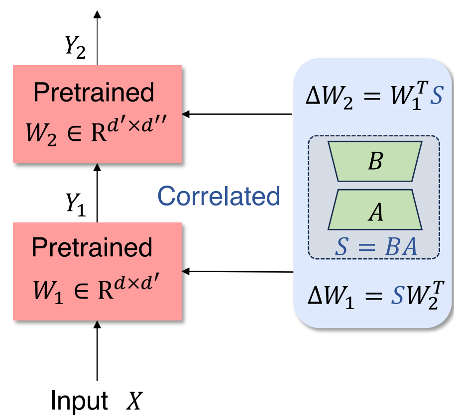
(c) Correlated-LoRA ( Ours )
